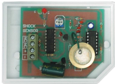
Shock Sensor
